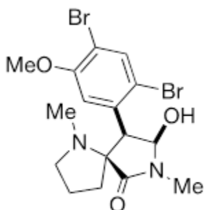
amathaspiramide A
